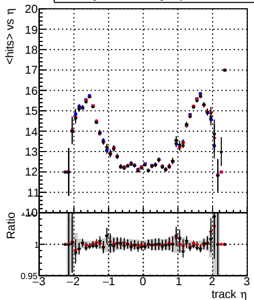
mean hits vs \eta DQM_TT_mkFit-DQM_original-0 DQM_TT_mkFit-DQM_original-127 DQM_TT_mkFit-DQM_updated-127
