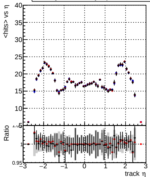
mean hits — DQM_TT_mkFit-DQM_original-0 — DQM_TT_mkFit-DQM_original-127 — DQM_TT_mkFit-DQM_updated-127
