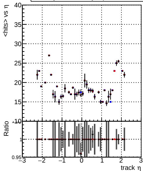
mean hits DQM_TT_mkFit-DQM_original-0 DQM_TT_mkFit-DQM_original-127 DQM_TT_mkFit-DQM_updated-127
