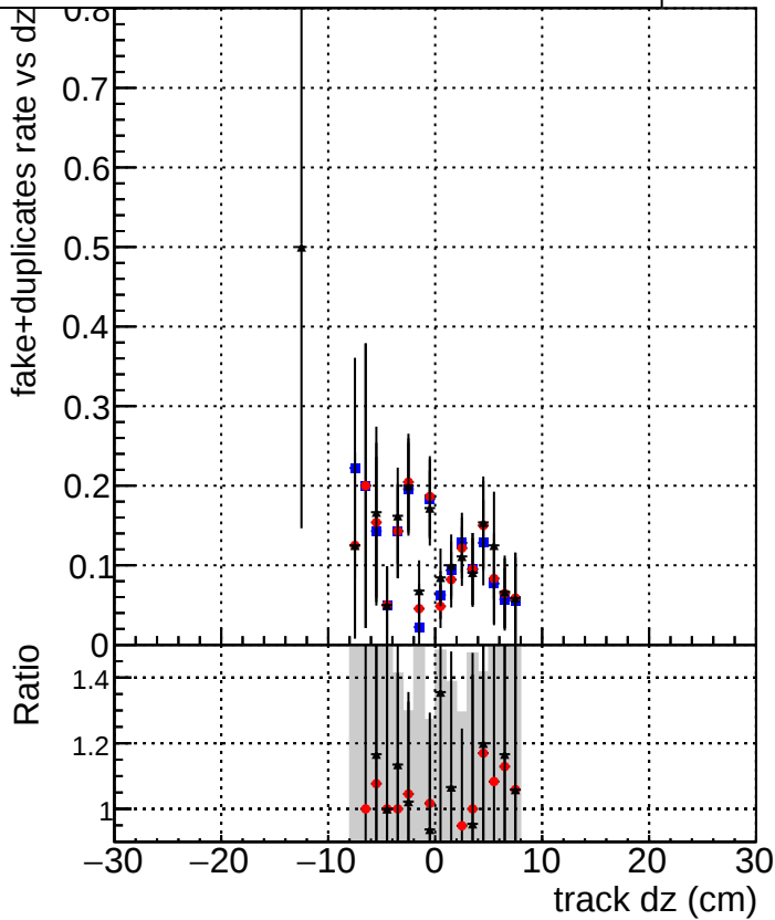
Legend for the bottom plot: DQM_TT_mkFit-DQM_original-0 (Blue squares) DQM_TT_mkFit-DQM_original-127 (Red circles) DQM_TT_mkFit-DQM_updated-127 (Black triangles)
