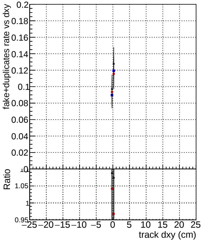
Legend for the bottom plot: DQM_TT_mkFit-DQM_original-0 (Blue squares) DQM_TT_mkFit-DQM_original-127 (Red circles) DQM_TT_mkFit-DQM_updated-127 (Black triangles)
