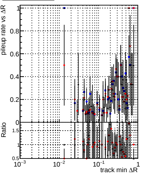
Legend: DQM TT mkFit-DQM original-0 (blue dots), DQM TT mkFit-DQM original-127 (red dots), DQM TT mkFit-DQM updated-127 (black dots with error bars)
