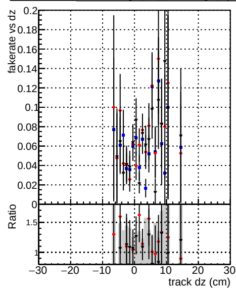
Legend for Fake rate vs d, Duplicates Rate vs Dxy, and Pileup rate vs dxy plots: DOM TT mkFit-DOM original-0 DOM TT mkFit-DOM original-127 DOM TT mkFit-DOM updated-127
