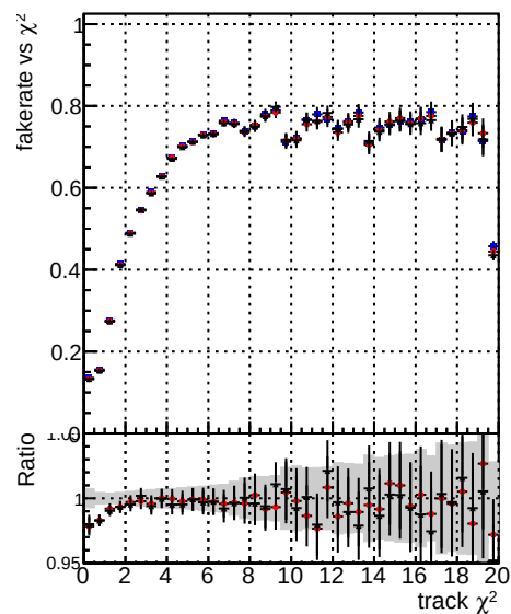
Fake rate vs. Legend Line Style Color Series DOM TT Blue Point mkFit-DOM original-0 DOM TT Red Point mkFit-DOM original-127 DOM TT Black Line mkFit-DOM updated-127
