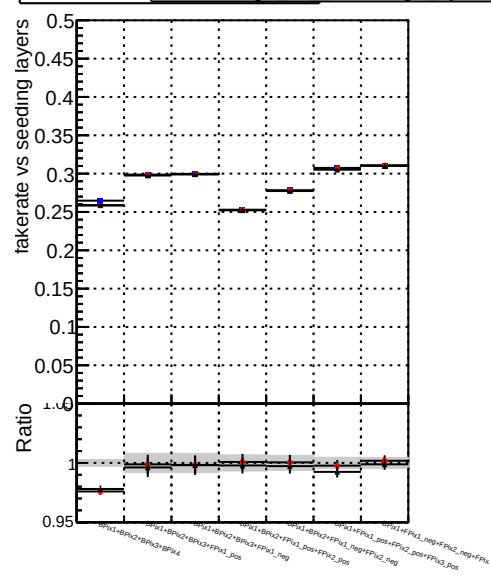
Fake rate vs. Legend Line Style Color Series DOM TT Blue Point mkFit-DOM original-0 DOM TT Red Point mkFit-DOM original-127 DOM TT Black Line mkFit-DOM updated-127
