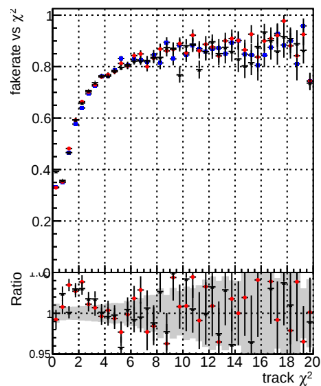
Fake rate vs. Series Color Shape DOM TT Black Circle mkFit-DOM original-0 Blue Circle mkFit-DOM original-127 Red Circle
