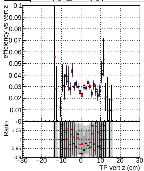
Efficiency vs. TP vert z (cm) — DQM_TT_mkFit-DQM_original-0 — DQM_TT_mkFit-DQM_original-127 — DQM_TT_mkFit-DQM_updated-127
