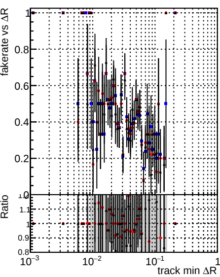
Legend: DQM TT mkFit-DQM original-0 (black), DQM TT mkFit-DQM original-127 (red), DQM TT mkFit-DQM updated-127 (blue)
