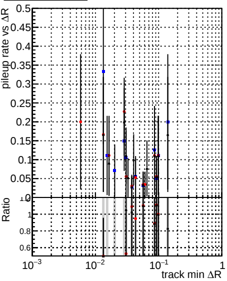
Legend: DQM TT mkFit-DQM original-0 (black), DQM TT mkFit-DQM original-127 (red), DQM TT mkFit-DQM updated-127 (blue)
