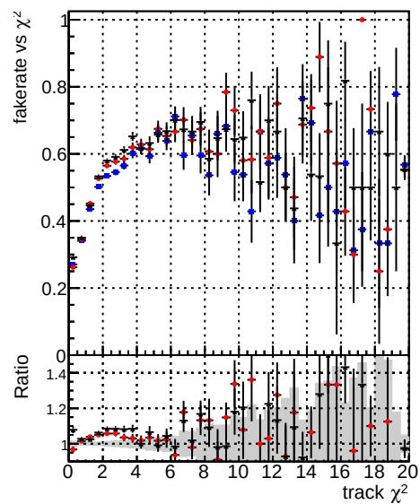
Fake rate vs. — DOM TT mkFit-DOM original-0 — DOM TT mkFit-DOM original-127 — DOM TT mkFit-DOM updated-127
