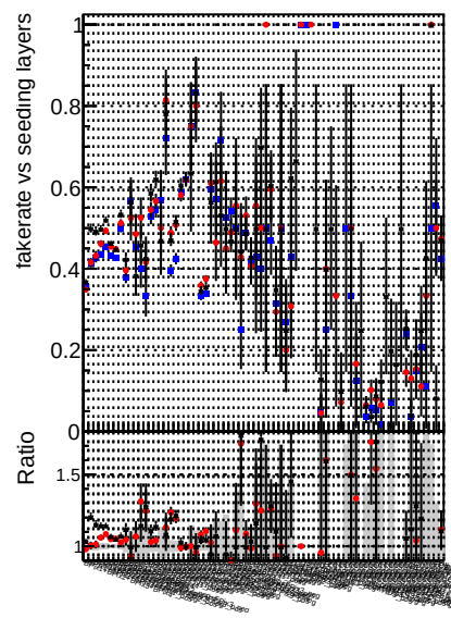
Fake rate vs. — DOM TT mkFit-DOM original-0 — DOM TT mkFit-DOM original-127 — DOM TT mkFit-DOM updated-127
