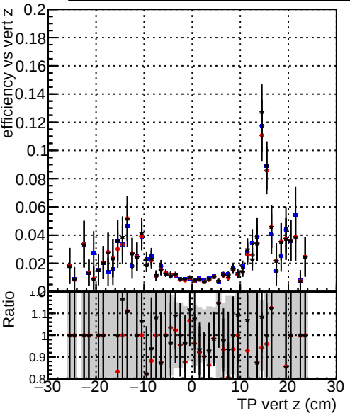
Efficiency vs vertpos Legend: DQM_TT_mkFit-DQM_original-0 DQM_TT_mkFit-DQM_original-127 DQM_TT_mkFit-DQM_mod-127
