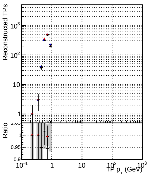
Legend for all plots: DQM_TT_mkFit-DQM_original-0 (Blue circles) DQM_TT_mkFit-DQM_original-127 (Red circles) DQM_TT_mkFit-DQM_mod-127 (Black circles)
