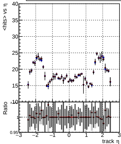
mean hits — DQM_TT_mkFit-DQM_original-0 — DQM_TT_mkFit-DQM_original-127 — DQM_TT_mkFit-DQM_mod-127
