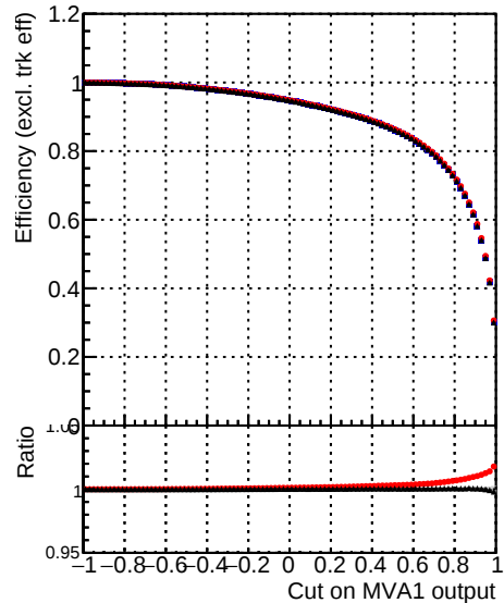
Efficiency (tracking eff factorized out) vs. MVA1
