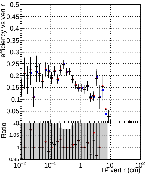
Efficiency vs TP vert r (cm) Legend: DQM_TT_mkFit-DQM_original-0 DQM_TT_mkFit-DQM_original-127 DQM_TT_mkFit-DQM_mod-127
