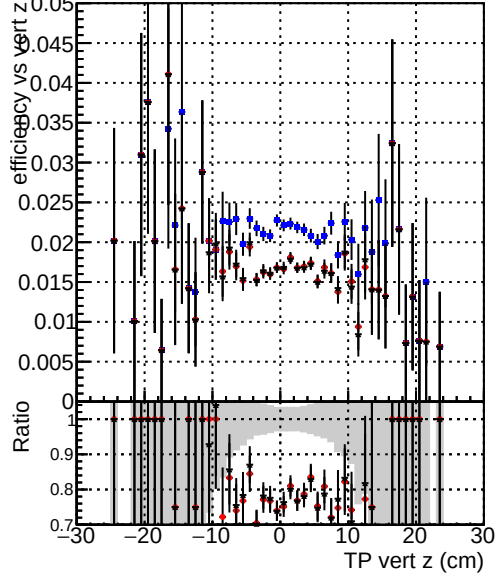
Efficiency vs vertpos — DQM_TT_mkFit-DQM_original-0 — DQM_TT_mkFit-DQM_original-127 — DQM_TT_mkFit-DQM_mod-127
