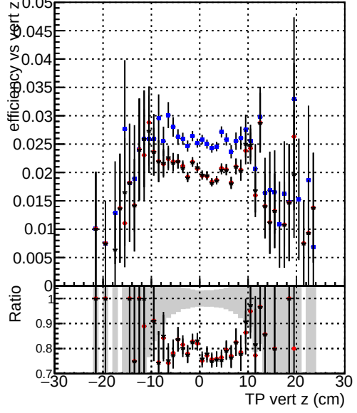
Efficiency vs. TP vert z (cm) — DQM_TT_mkFit-DQM_original-0 — DQM_TT_mkFit-DQM_original-127 — DQM_TT_mkFit-DQM_mod-127
