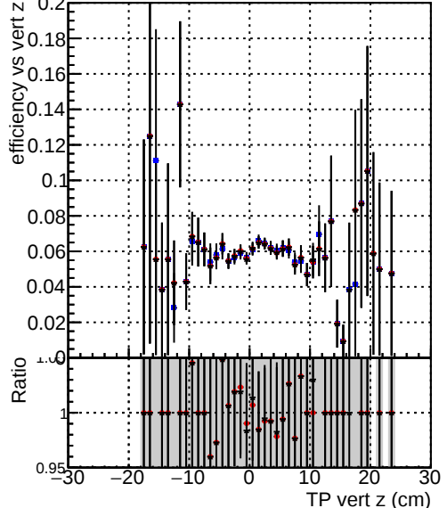
—●— DQM_TT_mkFit-DQM_original-0 —●— DQM_TT_mkFit-DQM_original-127 —●— DQM_TT_mkFit-DQM_mod-127
