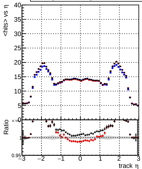
DQM_TT_mkFit-DQM_original-0 DQM_TT_mkFit-DQM_original-127 DQM_TT_mkFit-DQM_mod-127 mean hits
