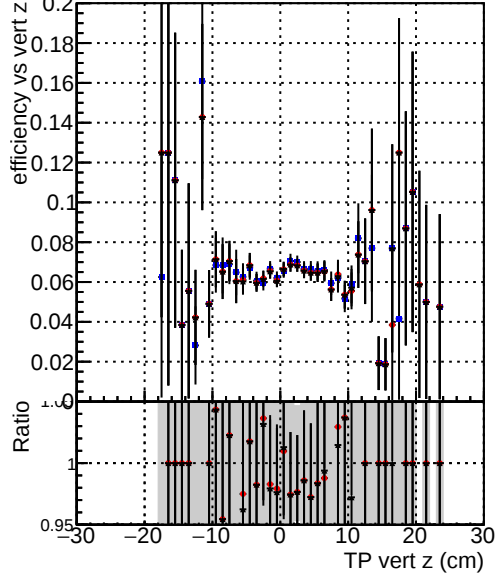
Efficiency vs. sim PV z —●— DQM_TT_mkFit-DQM_original-0 —●— DQM_TT_mkFit-DQM_original-127 —●— DQM_TT_mkFit-DQM_mod-127
