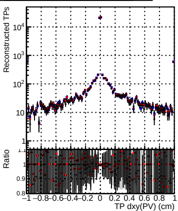
Legend: DQM_TT_mkFit-DQM_original-0 DQM_TT_mkFit-DQM_mod-127 DQM_TT_mkFit-DQM_mod_updatedmod-127
