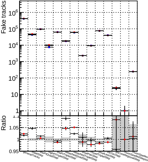
Number ● DQM_TT_mkFit-DQM_mod-127 ▲ DQM_TT_mkFit-DQM_mod_updatedmod-127
