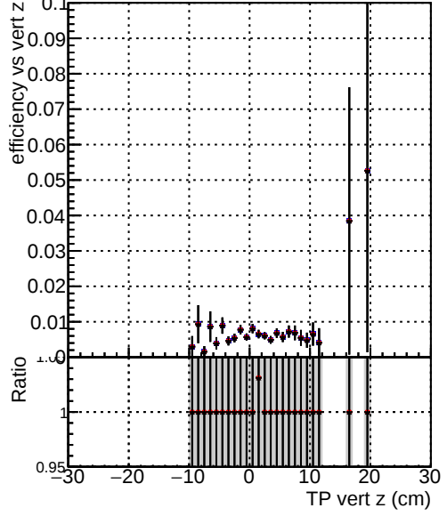
Efficiency vs. TP vert z (cm) —●— DQM_TT_mkFit-DQM_original-0 —●— DQM_TT_mkFit-DQM_mod-127 —●— DQM_TT_mkFit-DQM_mod_updatedmod-127
