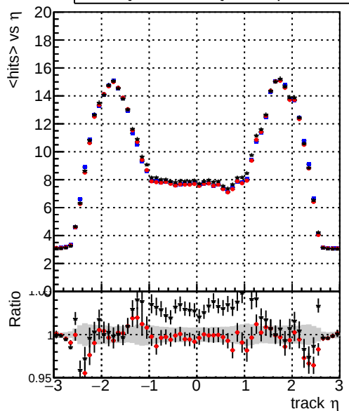
mean hit — DQM_TT_mkFit-DQM_original-0 — DQM_TT_mkFit-DQM_mod-127 — DQM_TT_mkFit-DQM_mod_updatedmod-127
