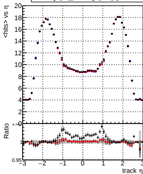
DQM_TT_mkFit-DQM_original-0 DQM_TT_mkFit-DQM_mod-127 DQM_TT_mkFit-DQM_mod_updatedmod-127 mean hit
