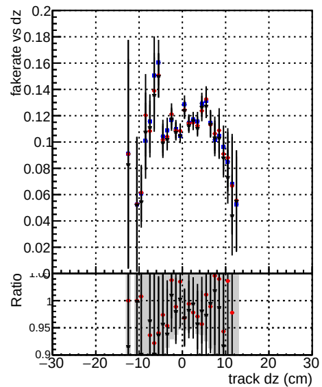
Fake rate vs dz Legend: DOM TT mkFit-DOM-original-0 DOM TT mkFit-DOM-mod-127 DOM TT mkFit-DOM-mod-updatedmod-127
