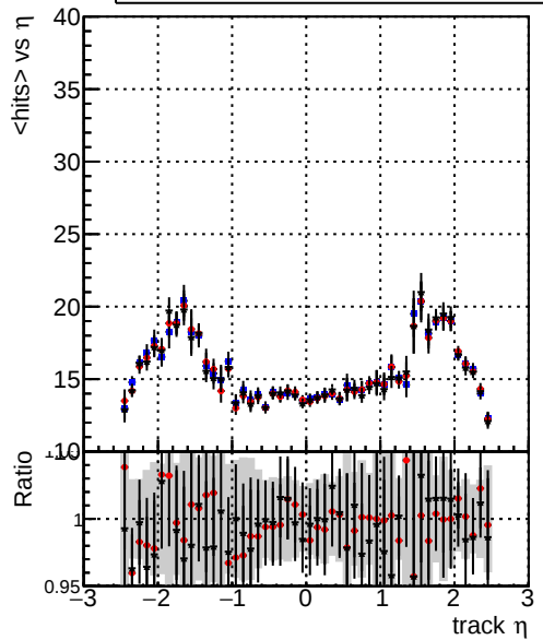
mean hits — DQM_TT_mkFit-DQM_original-0 — DQM_TT_mkFit-DQM_mod-127 — DQM_TT_mkFit-DQM_mod_updatedmod-127
