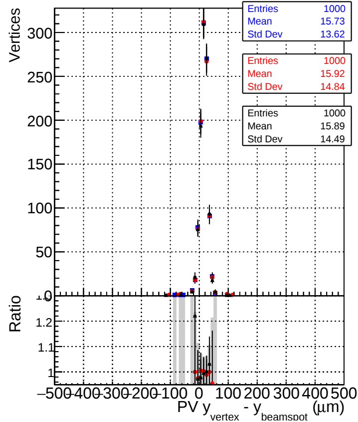
Y distance from BeamSpot (tagged vtx)
