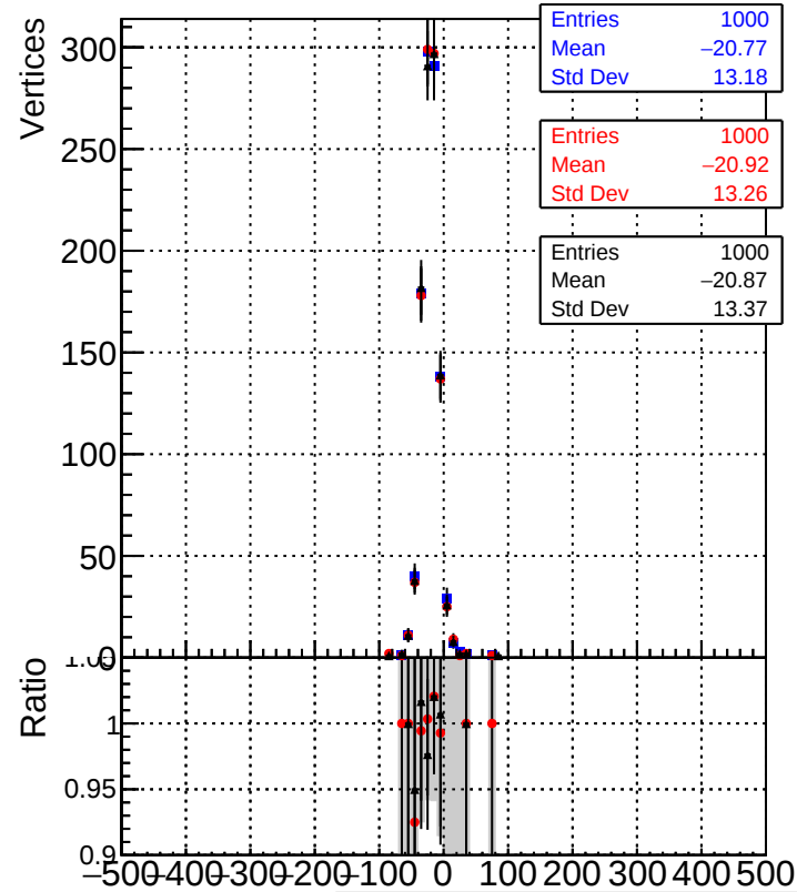
X distance from BeamSpot (tagged Vtx)
