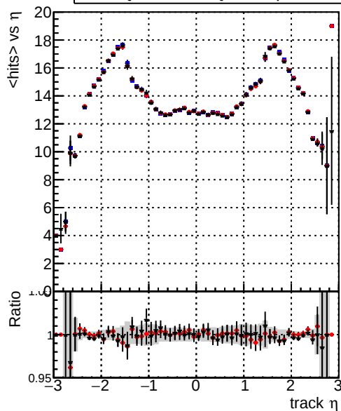
mean hit — DQM_TT_mkFit-DQM_original-0 — DQM_TT_mkFit-DQM_mod-127 — DQM_TT_mkFit-DQM_mod_updatedmod-127
