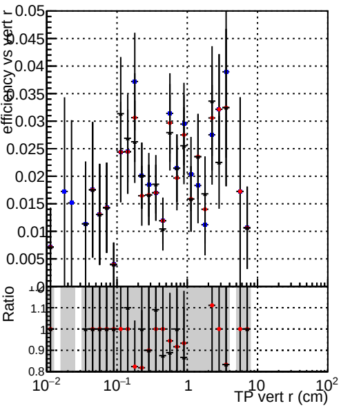
Efficiency vs TP vert r (cm) Legend: DQM_TT_mkFit-DQM_original-0 DQM_TT_mkFit-DQM_mod-127 DQM_TT_mkFit-DQM_mod_updatedmod-127
