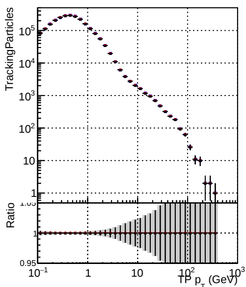
Legend for all plots: Blue line with circles: DQM_TT_mkFit-DQM_original-0 Red line with circles: DQM_TT_mkFit-DQM_mod-127 Black line with crosses: DQM_TT_mkFit-DQM_mod_updatedmod-127
