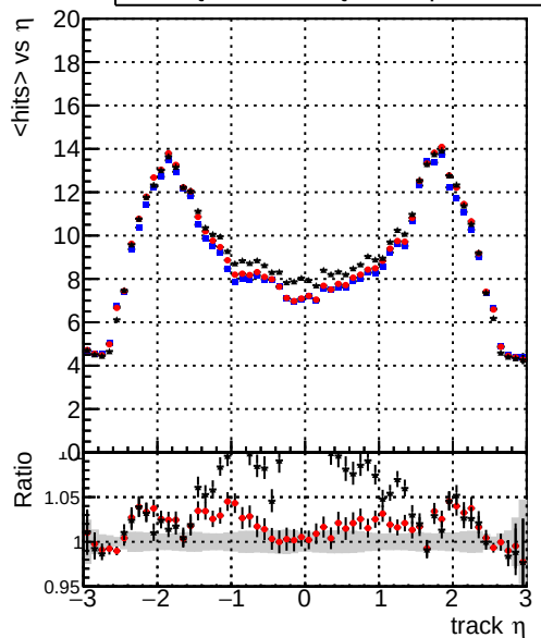
— DQM_TT_mkFit-DQM_original-0 — DQM_TT_mkFit-DQM_mod-127 — DQM_TT_mkFit-DQM_mod_updatedmod-127 mean hit
