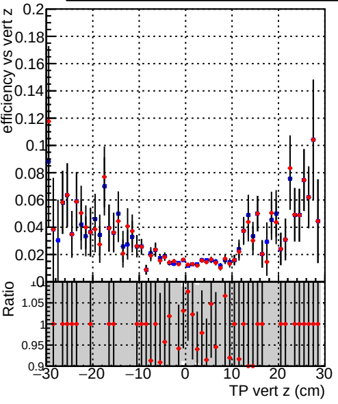
Efficiency vs vertpos Legend: DQM_TT_mkFit-DQM_original-0 DQM_TT_mkFit-DQM_original-127
