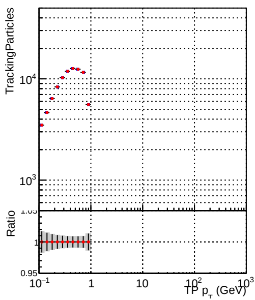
—●— DQM_TT_mkFit-DQM_original-0 —●— DQM_TT_mkFit-DQM_original-127
