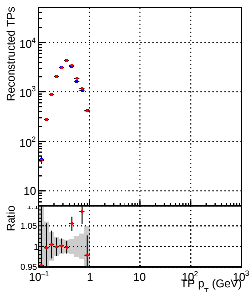
—●— DQM_TT_mkFit-DQM_original-0 —●— DQM_TT_mkFit-DQM_original-127
