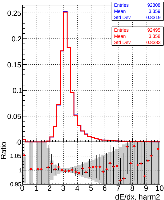
■ DQM_TT_mkFit-DQM_original-0 ● DQM_TT_mkFit-DQM_original-127
