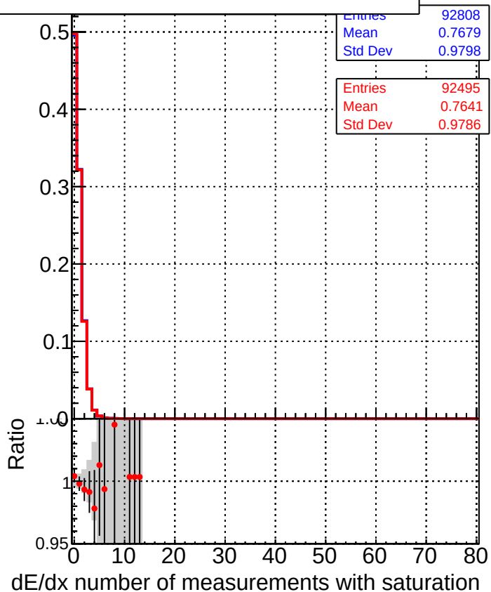
■ DQM_TT_mkFit-DQM_original-0 ● DQM_TT_mkFit-DQM_original-127
