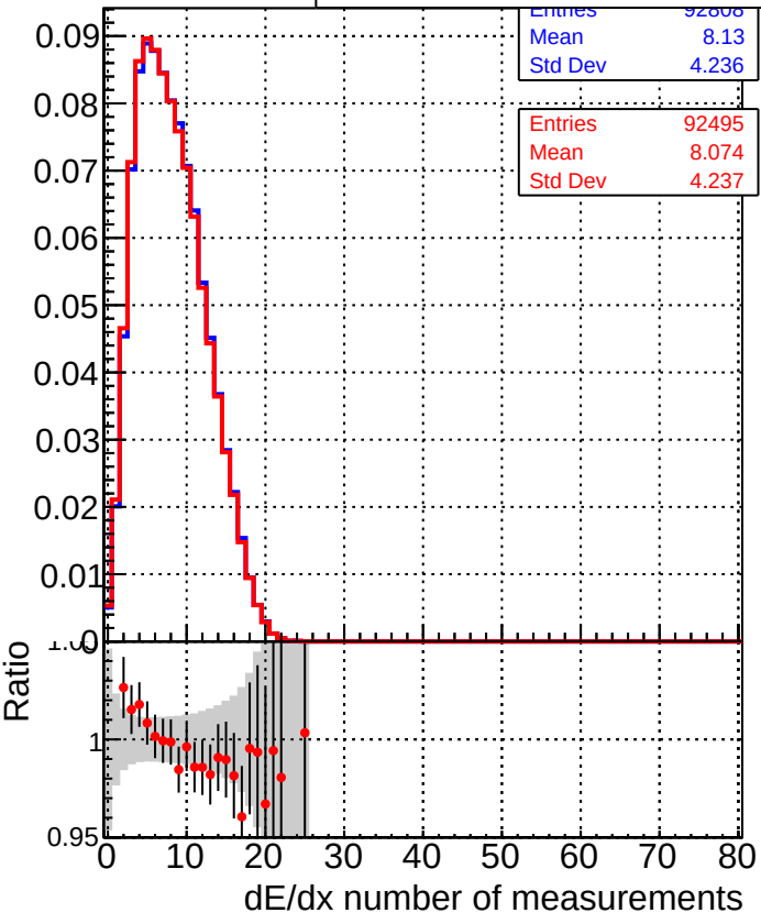
■ DQM_TT_mkFit-DQM_original-0 ● DQM_TT_mkFit-DQM_original-127
