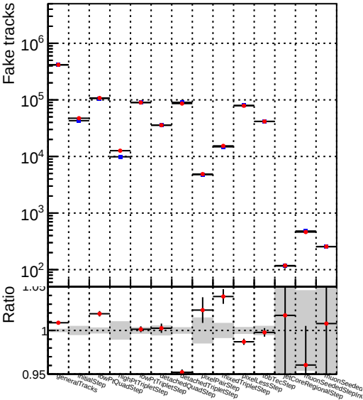
Number —●— DQM_TT_mkFit-DQM_original-127
