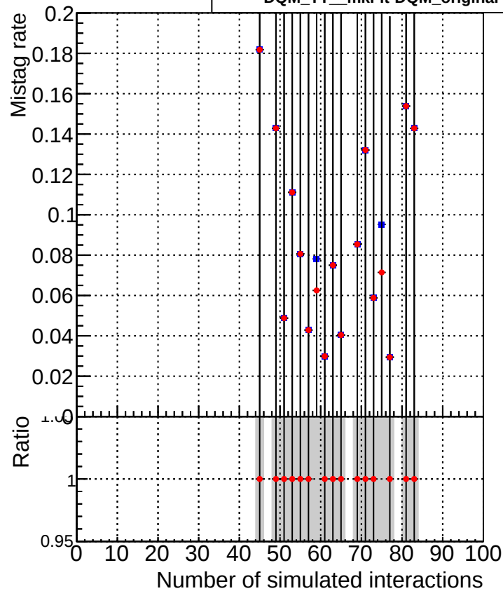
—■ DQM_TT_mkFit-DQM_original-0 —● DQM_TT_mkFit-DQM_original-127
