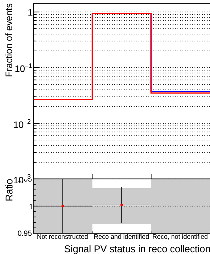
—■ DQM_TT_mkFit-DQM_original-0 —● DQM_TT_mkFit-DQM_original-127
