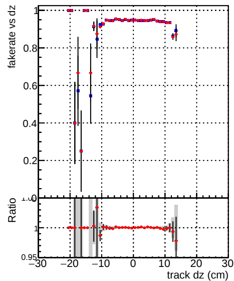
Fake rate vs dz —●— DQM_TT_mkFit-DQM_original-0 —●— DQM_TT_mkFit-DQM_original-127
