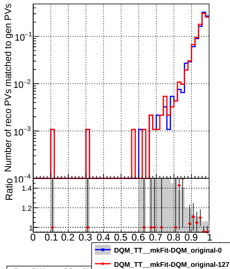
RecoPVAssoc2GenPVmatched_missing
