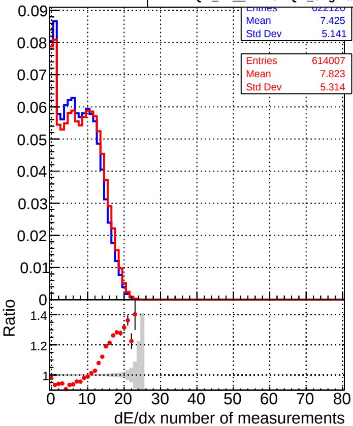
— DQM_TT_mkFit-DQM_original-0 — DQM_TT_mkFit-DQM_original-127
