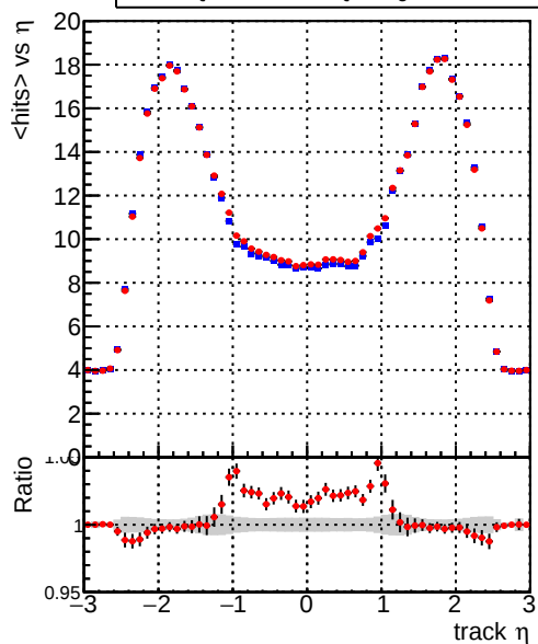
— DQM_TT_mkFit-DQM_original-0 — DQM_TT_mkFit-DQM_original-127
