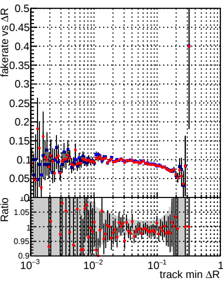
Legend: DQM_TT_mkFit-DQM_original-0 (blue line with error bars), DQM_TT_mkFit-DQM_original-127 (red line with error bars)
