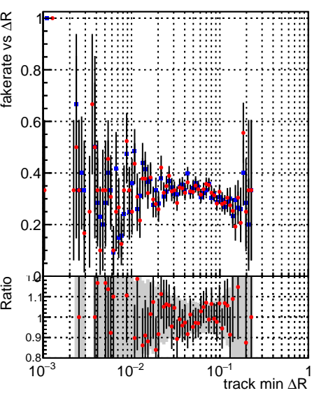
■ DQM_TT_mkFit-DQM_original-0 ● DQM_TT_mkFit-DQM_original-127
