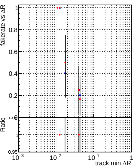
Fake rate vs ΔR(track, jet) DQM_TT_mkFit-DQM_original-0 DQM_TT_mkFit-DQM_original-127
