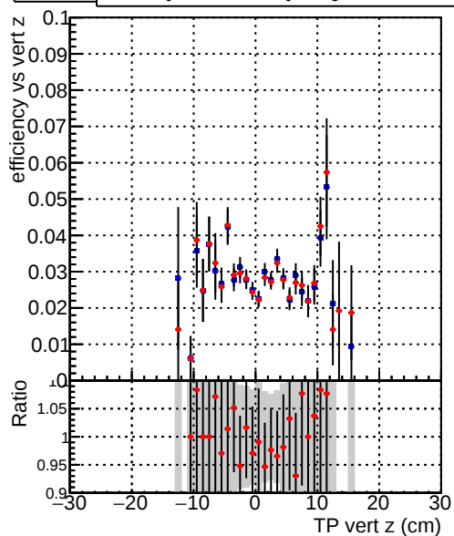
Efficiency vs. TP vert z (cm) — DQM_TT_mkFit-DQM_original-0 — DQM_TT_mkFit-DQM_original-127
