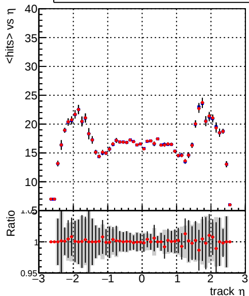
mean hits — DQM_TT_mkFit-DQM_original-0 — DQM_TT_mkFit-DQM_original-127
