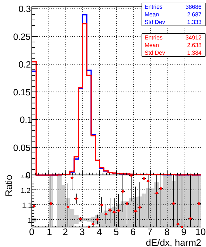
DQM_TT_mkFit-DQM_original-0 DQM_TT_mkFit-DQM_original-127
