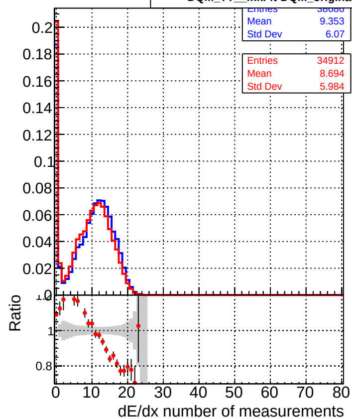
DQM_TT_mkFit-DQM_original-0 DQM_TT_mkFit-DQM_original-127
