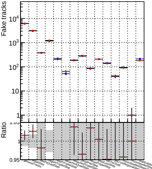
Number —●— DQM_TT_mkFit-DQM_original-127
