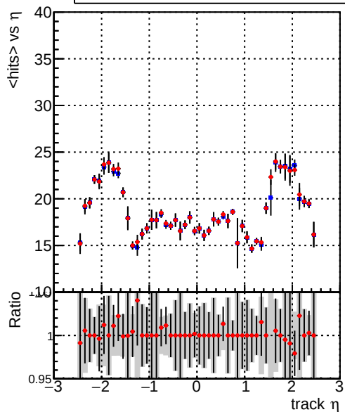
mean hits vs \eta Legend: DQM_TT_mkFit-DQM_original-0 (blue line with markers), DQM_TT_mkFit-DQM_original-127 (red line with markers)
